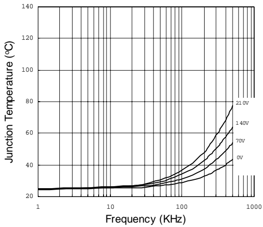
Figure 40. IR21094 vs Frequency (IRFBC40) Rgate = 15Ω, VCC = 15V
