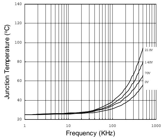
Figure 41. IR21094 vs Frequency (IRFPE50) Rgate = 10Ω, VCC = 15V
