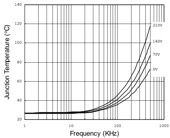
Figure 33. IR2109 vs Frequency (IRFPE50) R gate = 10Ω, V CC = 15V
