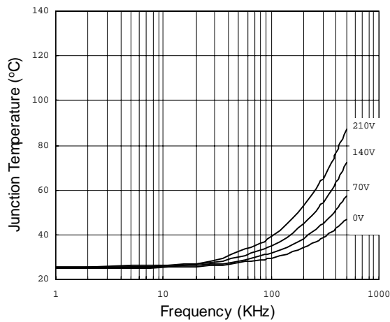
Figure 32. IR2109 vs Frequency (IRFBC40) R gate = 15Ω, V CC = 15V
