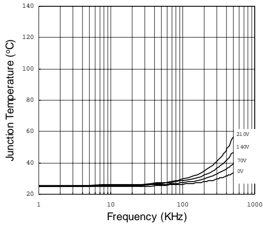
Figure 38. IR21094 vs Frequency (IRFBC20) Rgate = 33Ω, VCC = 15V
