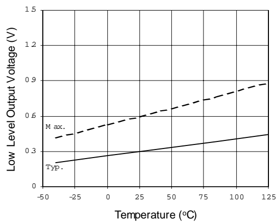
Figure 17A. Low Level Output Voltage vs. Temperature
