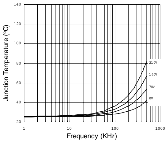
Figure 34. IR2109S vs Frequency (IRFBC20) R gate = 33Ω, V CC = 15V
