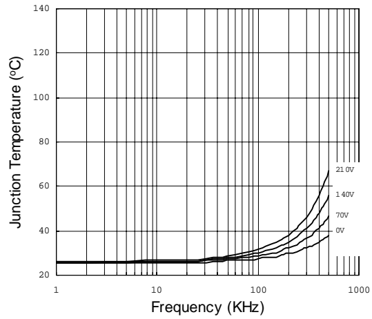
Figure 39. IR21094 vs Frequency (IRFBC30) Rgate = 22Ω, VCC = 15V
