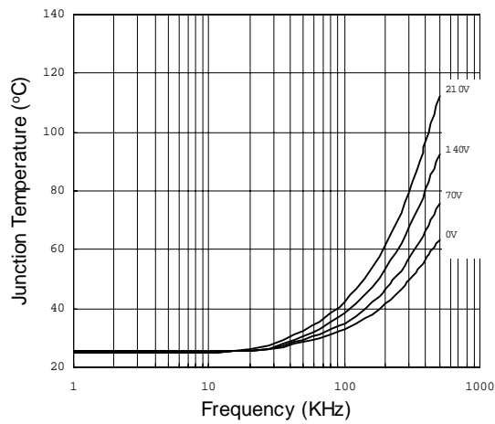
Figure 36. R2109S vs Frequency (IRFBC40) R gate = 15Ω, V CC = 15V
