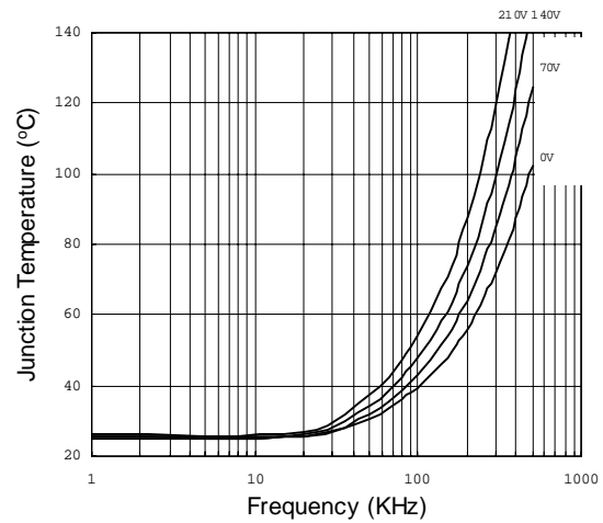
Figure 37. R2109S vs Frequency (IRFPE50) R gate = 10Ω, V CC = 15V
